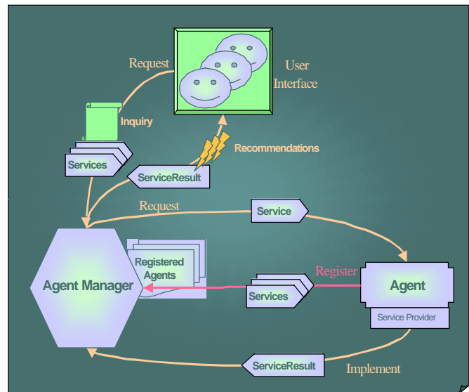
Figure 3. User Request
