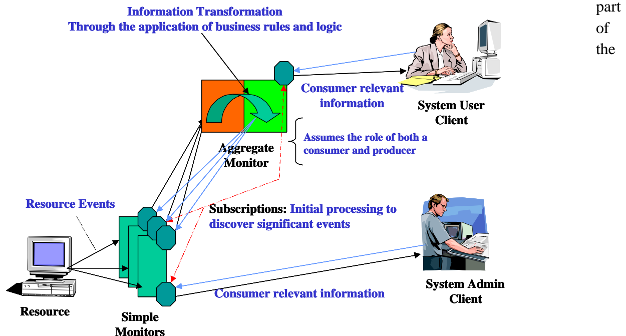
Figure 4: Monitors support multiple clients
