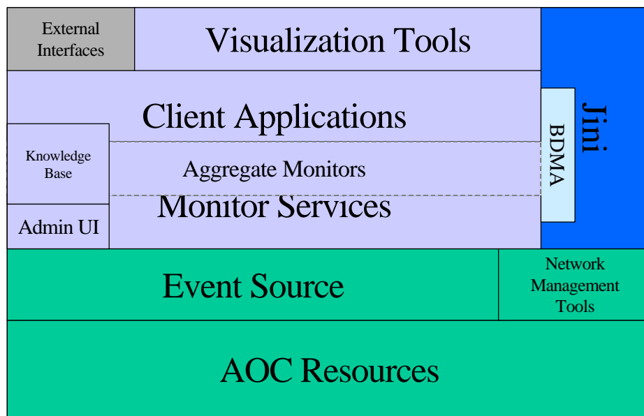
Figure 5: MCP Architecture
