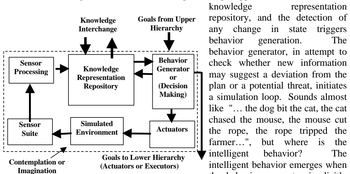
Figure 1. The Elementary Loop of Functioning (ELF)
