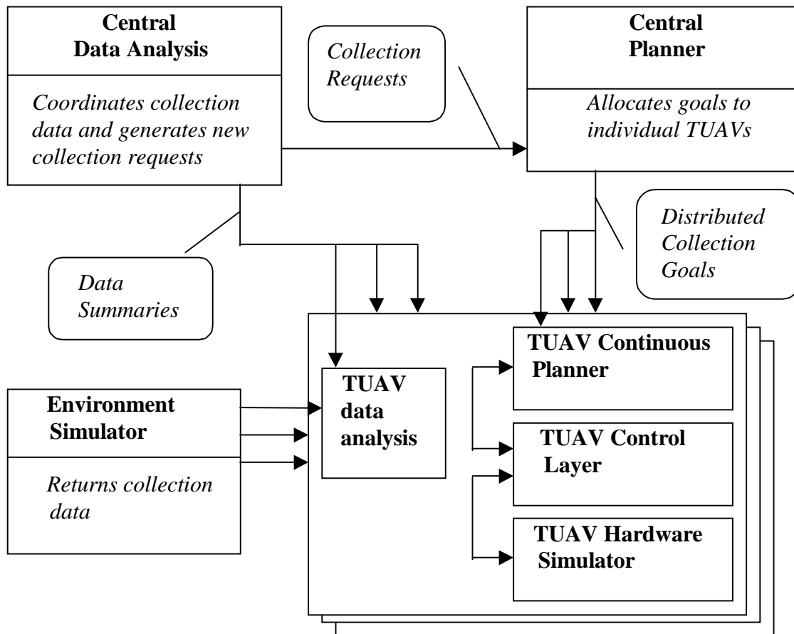
Figure 1. Multi-TUAV Execution Architecture
