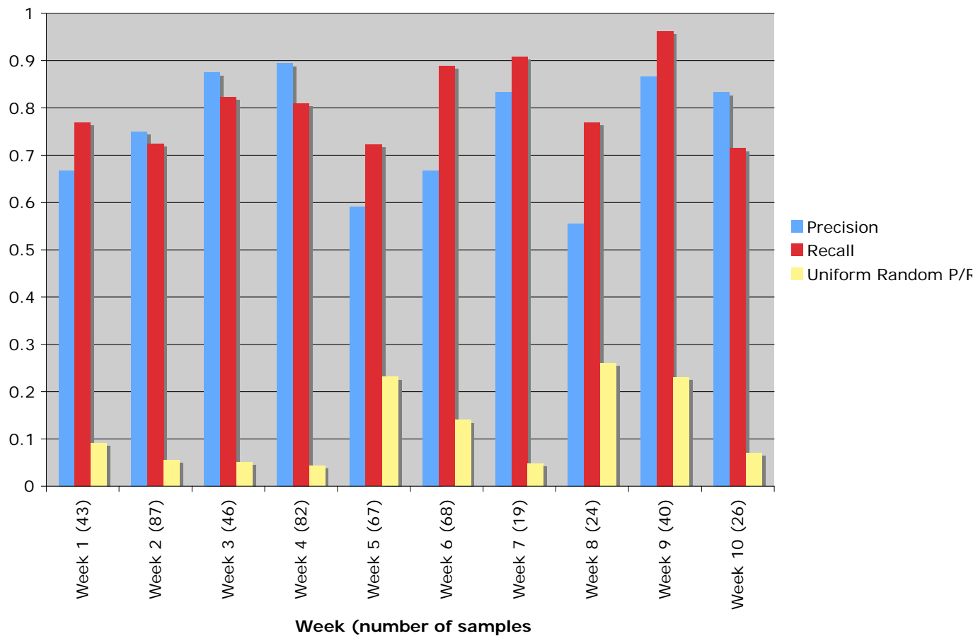
Score Threshold Scheme: Sampled Precision and Rec
